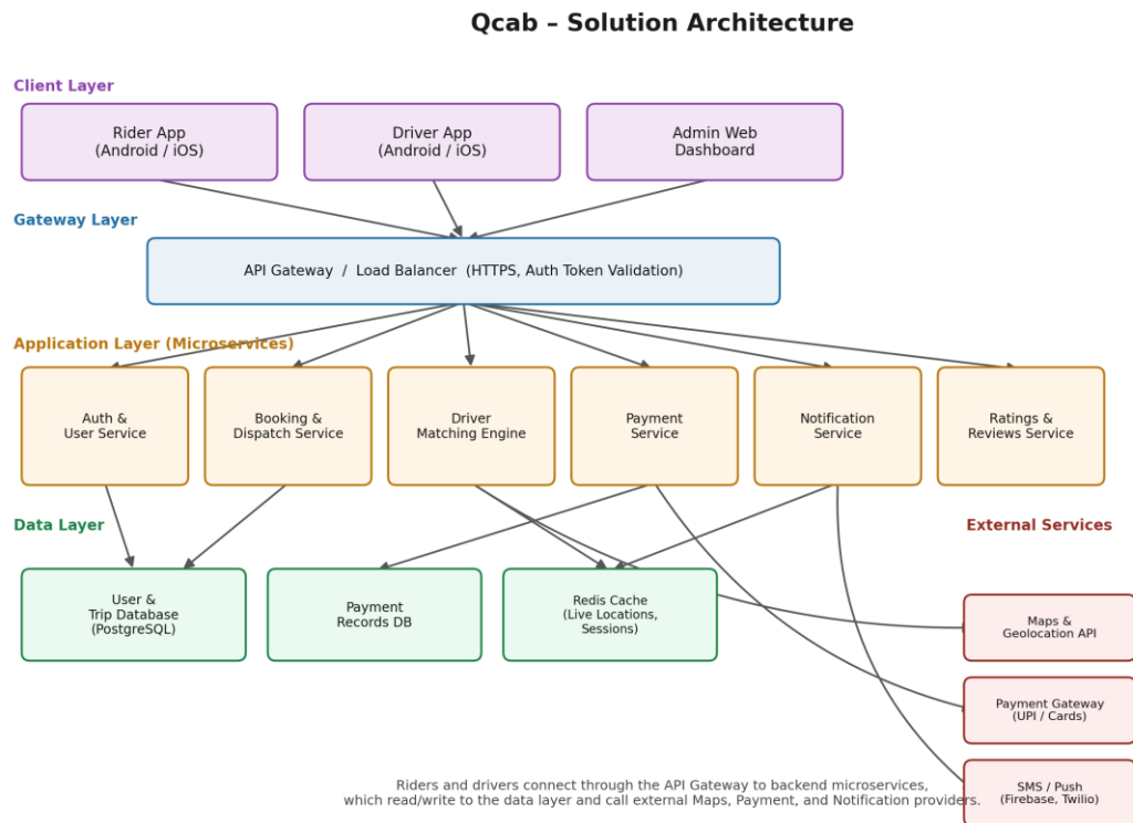
Figure 2: Qcab solution architecture – rider and driver apps connect via the API Gateway to backend microservices (Auth, Booking & Dispatch, Driver Matching, Payment, Notification, Ratings), which use the data layer and integrate with Maps, Payment Gateway, and SMS/Push notification providers.
